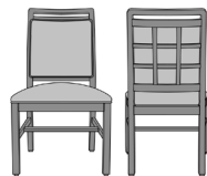
BLD04B1 24W 26.5D 40H
